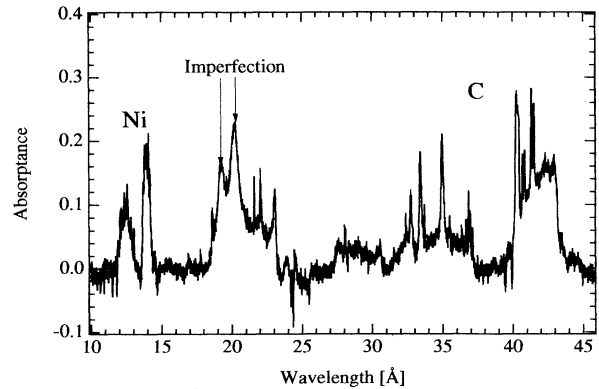
FIG. 2. The experimental spectrum includes contributions from C II to C V in the wavelength range 32–42 Å and a few ionization stages of Ni at wavelengths 12–14 Å. The features near 22 Å are of oxygen existing in the plastic layer not considered in this work. The features at 19–21 Å are imperfections in the photographic emulsion that appear in this particular lineout.
