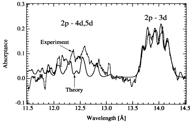
FIG. 5. The complete Ni LTE spectrum at T=14 eV + 18 eV and density 0.01 g/cc.
