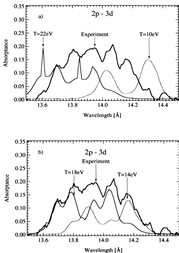
FIG. 3. Comparison between the theoretical and the experimental 2p \rightarrow 3d spectrum. (a) Two temperature (10 and 22 eV) spectra beyond the experimental limit. (b) The theoretical spectra of the temperature bounds (14 and 18 eV) reproducing the experimental spectrum.
