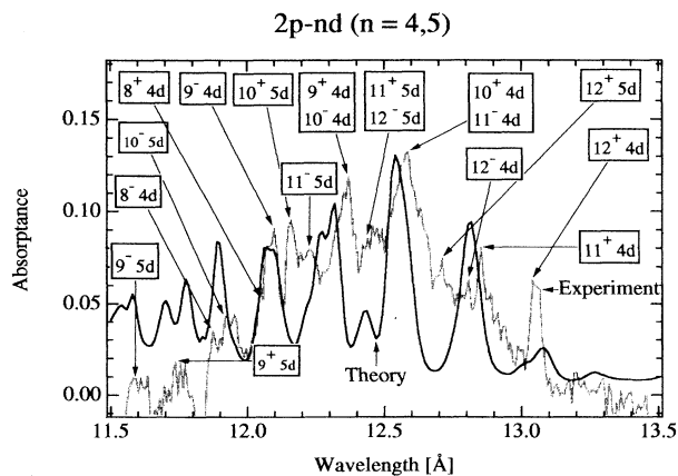
FIG. 6. Identification of the 2p\rightarrow 4d, 5d transitions. ( N, nl ) indicates the 2p\rightarrow nl one-electron jump origination from the bulk of superconfigurations denoted in the text by N , ( N, M : summed over all M ) of Eq. (13).
