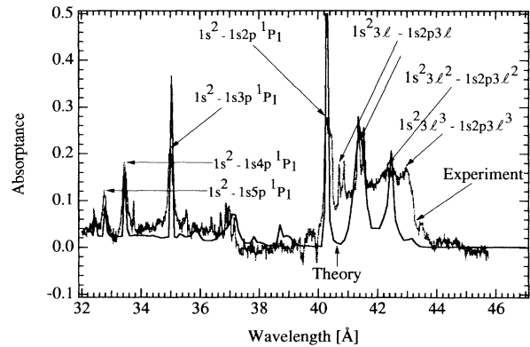
FIG. 7. Identification of the carbon LTE spectrum at T=14 eV + 18 eV and density 0.01 g/cc. The noisy and smooth lines are the experimental and theoretical results, respectively.
