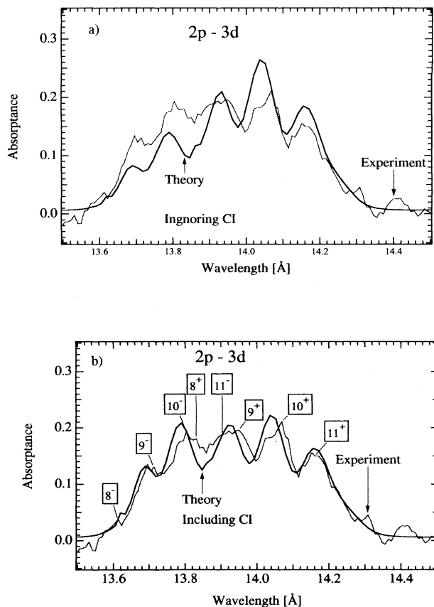
FIG. 4. The total two temperature (40% T=14 eV + 60% T=18 eV) spectra of 2p \rightarrow 3d : (a) without CI, and (b) with CI. N^+ and N^- indicate the 2p_{1/2} \rightarrow nd_{3/2} and 2p_{3/2} \rightarrow nd_{5/2} transitions, respectively.
